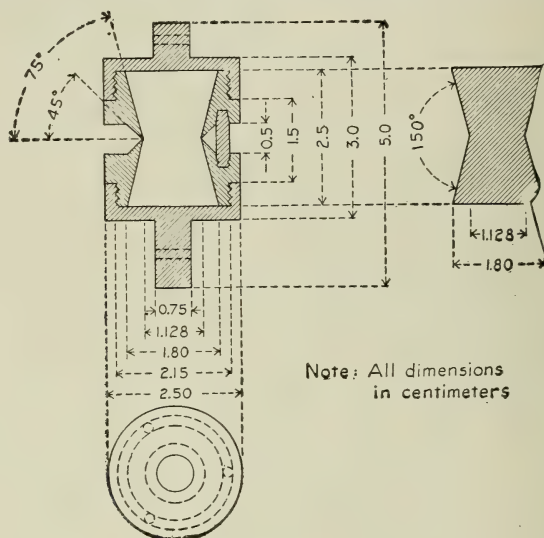
FIG. 169.—Cross-section Author's Mould.
